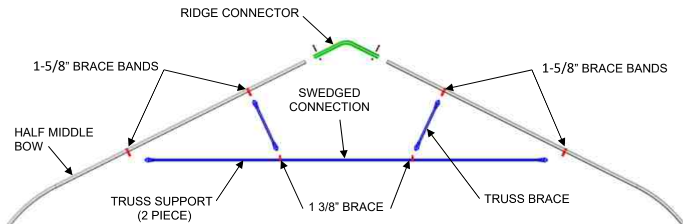
BOW ASSEMBLY (EXPLODED VIEW)
